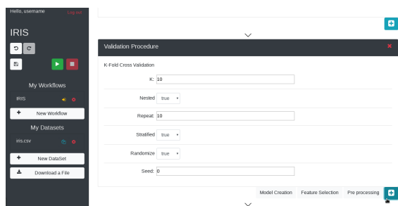
Figure 2: UI - Showing cross validation task (a validation procedure task) and the tasks that can be used after.
