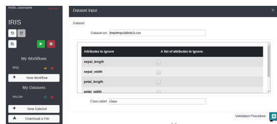
Figure 1: User interface - showing a dataset insertion task and the option to insert a validation procedure after clicking the plus button.
