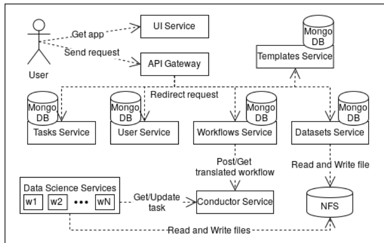
Figure 3: Current system's architecture.
