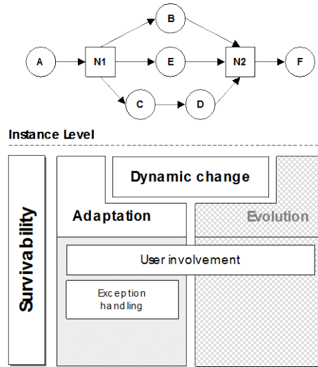
Figure 2 - Survivability architecture (adaptation and evolution) at the instance level
