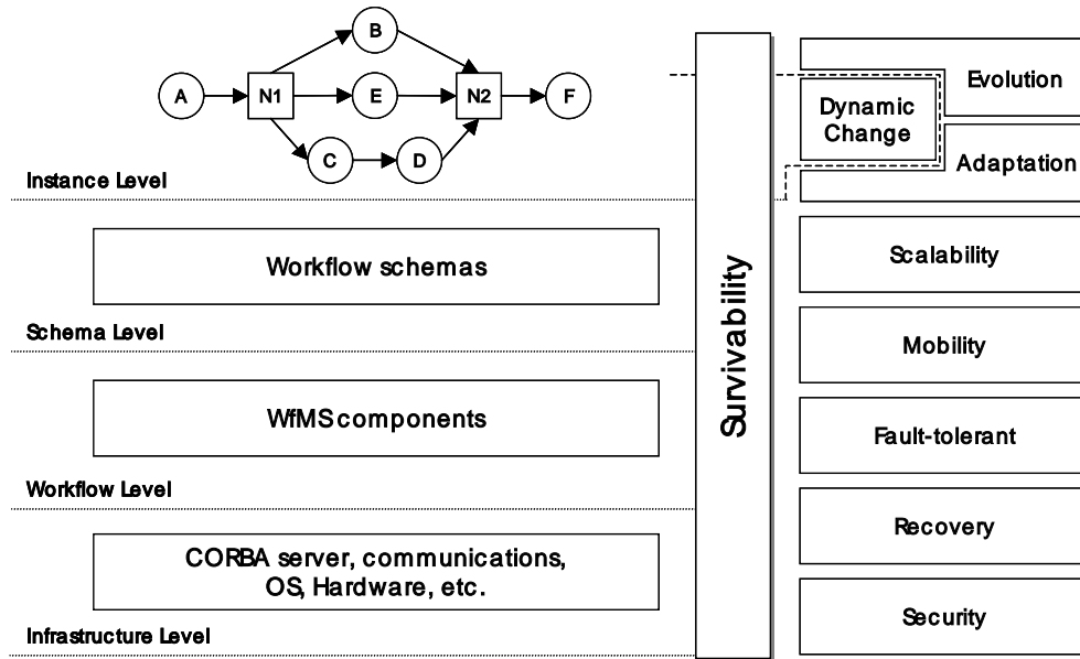
Figure 1- Survivability architecture for Workflow Management Systems
