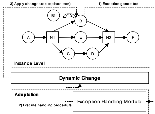
Figure 3 - Example of adaptation using Exception Handling mechanism
